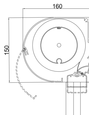
Zipscreen R 160 x 150
