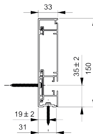
Kompriband (lose)
